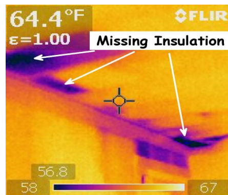
Thermal Imaging Infrared Inspection Information on pgs. 39 - 42
